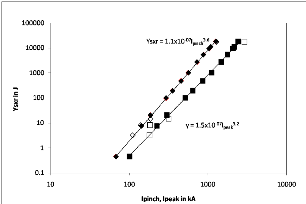
Figure 6. Y_{sxr} is plotted as a function of I_{pinch} and I_{peak} . The parameters kept constant for the black data points are: RESF = 0.1 , c = 1.5 , L_0 = 30nH and V_0 = 20 kV and model parameters f_m, f_c, f_{mr}, f_{cr} at 0.06, 0.7, 0.16 and 0.7 respectively. The unblackened data points are for specific machines which have different values for the parameters c, L_0, V_0 and RESF .
