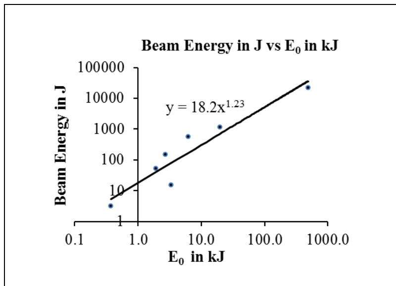
Figure 7. Establishing a first scaling law for deuteron beam energy in the plasma focus.
