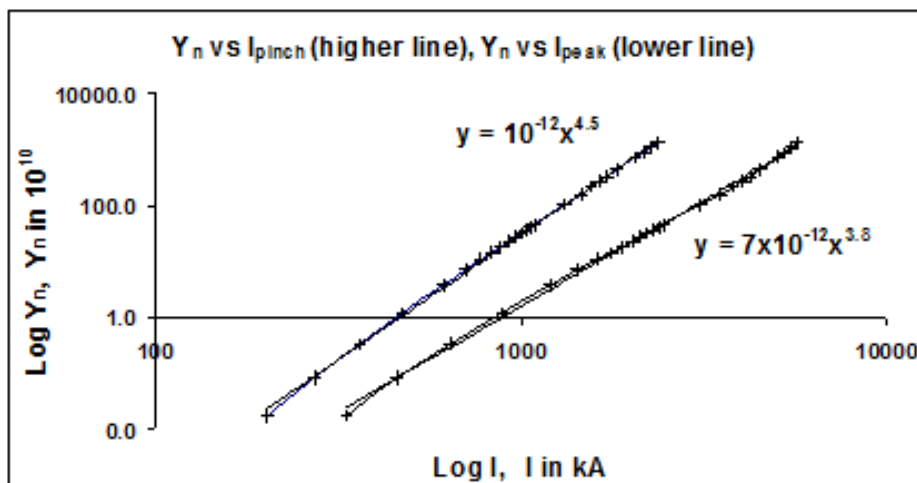
Figure 3. Log( Y_n ) scaling with log( I_{peak} ) and log( I_{pinch} ) for the range of energies up to 25 MJ.
